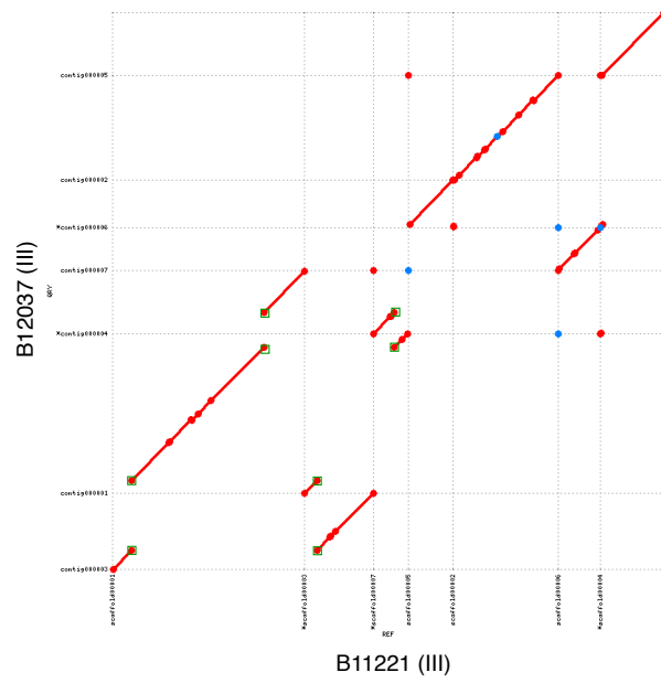
Supplementary Figure 6. Shared synteny regions based on whole genome alignments between C. auris B12037 and B11221. Green squares highlight translocation breakpoints.
