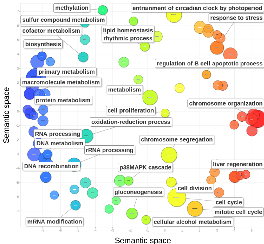
Figure S1. Enriched GO terms identified from genes with differential gene transcription between non-transgenic and transgenic coho salmon in a tank environment. GO terms complexity was reduced using Revigo software. Larger circles have lower p-values and the colour reflects semantic space. The x and y-axes are coordinates from multidimensional scaling of GO term semantic similarities into two dimensions.
