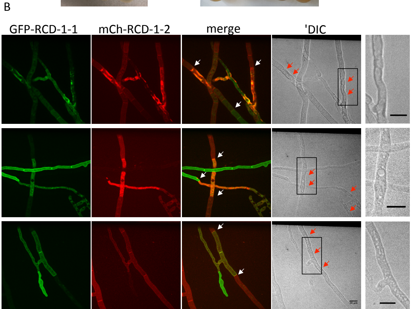
Figure S4. Heterokaryon incompatibility induced by RCD-1 allelic variants in hyphae of N. crassa . A. Germinating ascospores co-expressing rcd-1-1 and rcd-1-2 alleles show growth arrest approximately 24 hrs after germination and progressive melanization (over a period of 10 days). B. Hyphal fusion between strains expressing GFP-RCD-1-1 and mCherry-RCD-1-2 resulted in vacuolization and cellular death (red arrowheads) and cytoplasmic mixing restriction by compartmentation (white arrowheads). Black boxes indicate image crop position. Scale bars are 10 \mu m.
