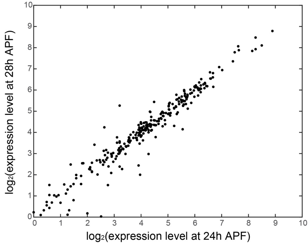
Supplemental Figure 1: Correlation of gene expression levels in male terminalia at 24h and 28h APF. For transcription factors expressed at levels greater than 1 read per kilobase per million reads (rpkm) at 28h after puparium formation (APF), we plotted log-transformed average expression levels at 28h APF versus log-transformed expression levels at 24h APF. The Pearson correlation coefficient for this data was 0.962.
