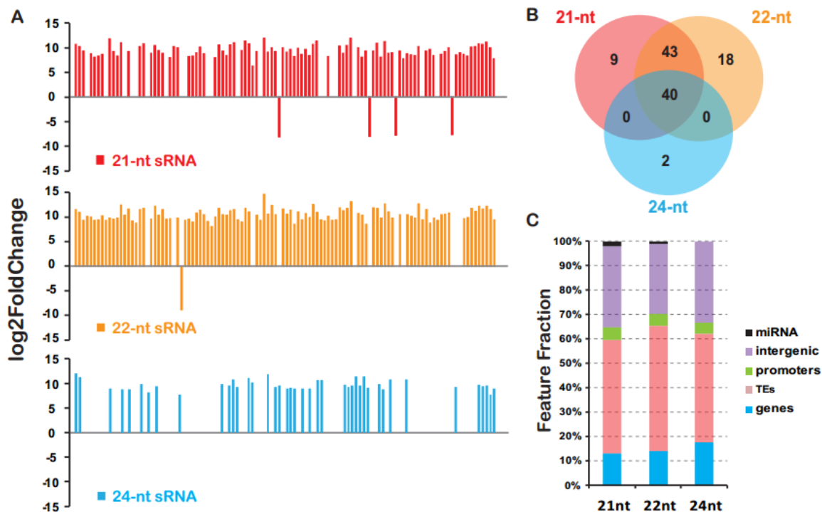
Figure S15. Feature analyses of differentially expressed sRNA regions between the sickly Bravo BC plants and the normal plants of B73 background. (A) Distribution of differentially expressed sRNA regions one-by-one that display a strong directional bias. Almost all of these differentially expressed sRNA regions produced increased 21-nt, 22-nt, and 24-nt sRNA in sickly plants compared to normal plants. The y-axis indicates the log2 transformation of fold changes, with positive value representing that increased sRNA were generated in sickly Bravo BC plants compared to the normal plants of B73 background. (B) Almost half of differentially expressed sRNA regions with increased sRNA in sickly plants produced three classes (21-nt, 22-nt, and 24-nt) of sRNAs concurrently. (C) Overlap profiling of differentially expressed sRNA regions with B73 genomic features, including genes, transposable elements (TEs), 2-kb promoter regions of annotated genes, and intergenic regions. The log2 fold change >0 means that increased sRNA were generated in sickly Bravo BC plants compared with the normal plants of B73 background. The log2 fold change <0 means that reduced sRNA were produced in sickly Bravo BC plants compared with the normal plants of B73 background.
