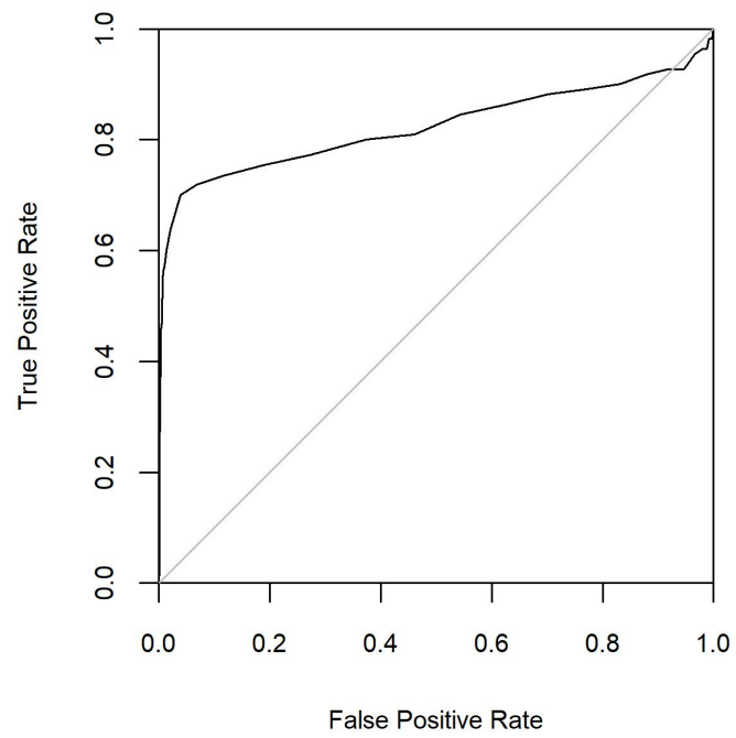
Figure S4 ROC curve for the auxotrophs we empirically identified, compared against those identified by Joyce et al. as the reference. TPRs and FPRs were calculated based on the median minimal media interaction score for the each of the auxotrophs we identified, at varying cutoffs. The AUC was 0.824.
