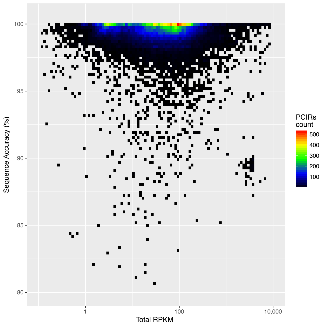
Figure S2: Evaluation of the impact of the expression level on Iso-Seq sequence accuracy. Density plot describing the distribution of PCIRs (polished-clustered Iso-Seq reads) based on the measured sequence accuracy and the cumulative expression value measured using RNA-seq.
