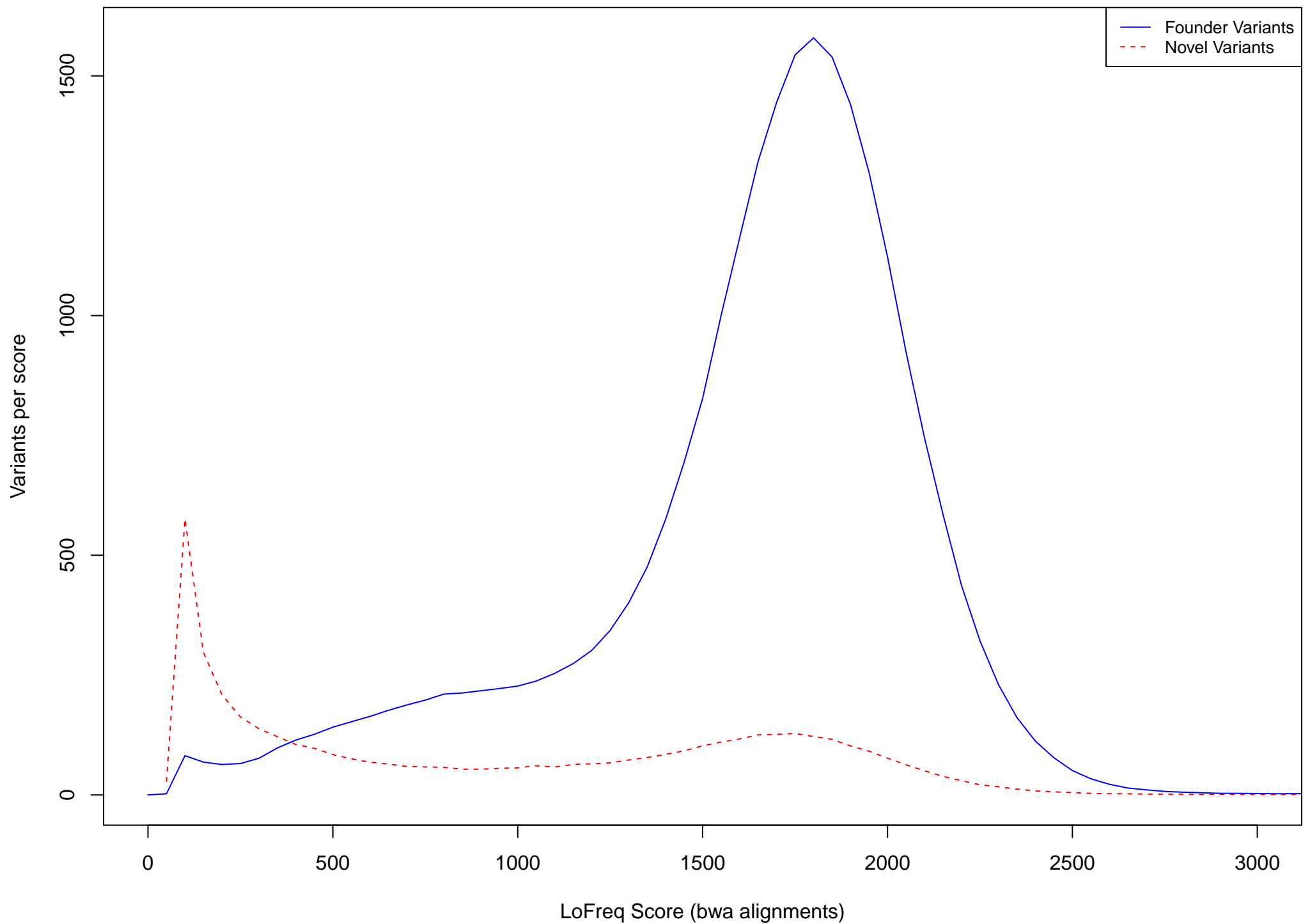
Figure S2. Plot of LoFreq score distributions for known and novel variants. The plot compares the scores of known DGRP variants versus novel variants detected by LoFreq.
